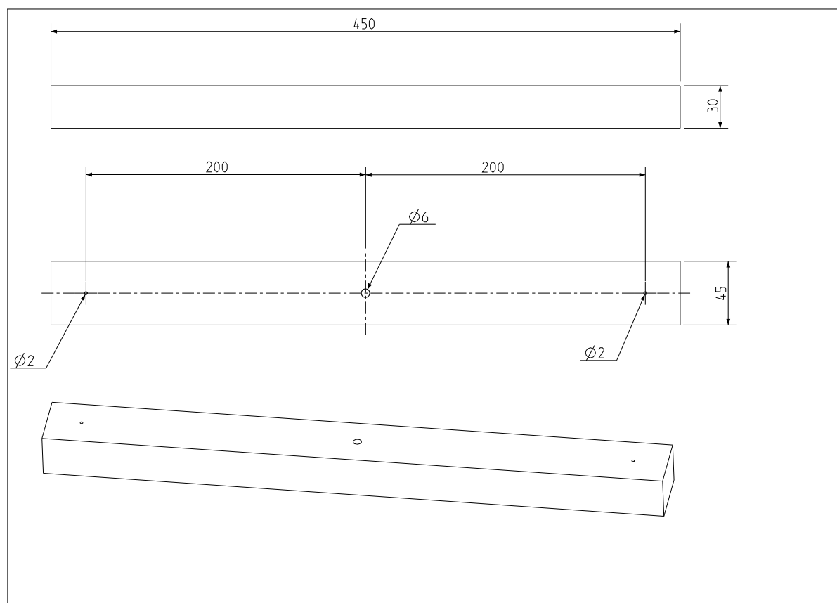
Figure 56 : Traverse
