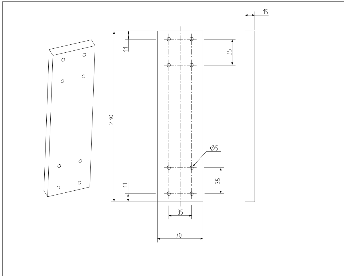
Figure 59 : Montants
